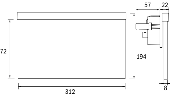
Maße AX Wandeinbaumontage Dimensions AX recessed wall mounted
