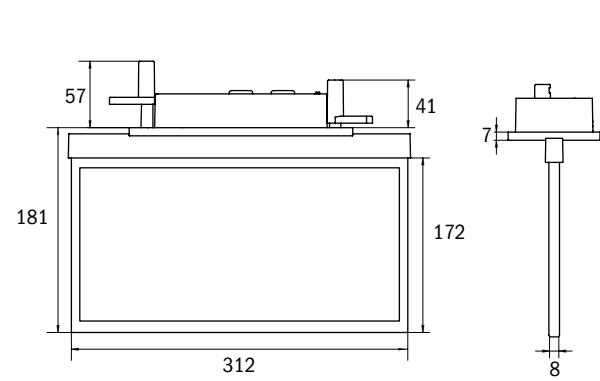
Maße AX Deckeneinbaumontage Dimensions AX recessed ceiling mounted
