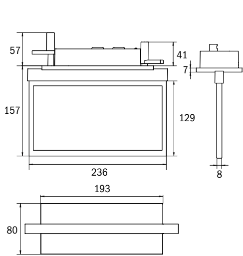
Maße AM Deckeneinbaumontage Dimensions AM recessed ceiling mounted
