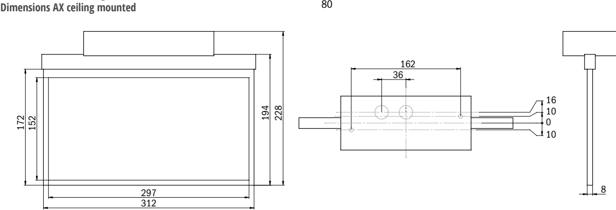
Maße AX Deckenmontage Dimensions AX ceiling mounted
